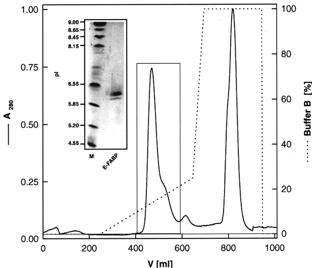
FIGURE 1: Anion-exchange chromatography on Q-Sepharose BB ( 20 \times 5 cm, 5 mL/min) as most effective step in the course of purification of recombinant human E-FABP (pooled fractions boxed). Buffer B, 1 M NaCl in 10 mM Tris-HCl (pH 7.4). (Inset) Microheterogeneity of recombinant human E-FABP (2 \mu g). Native isoelectric focusing was performed with PhastGel IEF gels (pI range 3–9) and pI markers (broad pI kit, pH 3.5–9.3, M).
