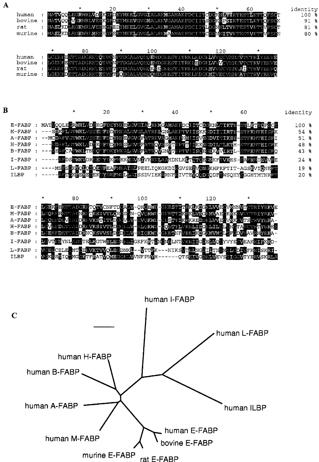
FIGURE 5: Amino acid alignment of E-FABP orthologs (A) and paralogs (B). Sequences were aligned using CLUSTAL W (implemented in the HUSAR 5.0 package, DKFZ Heidelberg, Germany) and displayed with GeneDoc 2.4.000 [Nicholas, K. B., and Nicholas, H. B., Jr. (1997). Distributed by the authors via http://www.cris.com/~ketchup/genedoc.shtml ]. Identical amino acids are shaded black and similar amino acids gray. Subfamilies are separated by a gap. (C) Radial rootless phylogenetic tree of mammalian E-FABP orthologs and paralogs. Subfamily of the cellular retinoid binding proteins (54) has been omitted for clarity. Phylogenetic order was calculated with CLUSTAL W and visualized by TreeView (55). Branch length represents evolutionary distance between proteins with the scale bar representing a substitution of 10 amino acids. GenBank accession numbers are (human E-FABP) M94856, (bovine E-FABP) U55188, (murine E-FABP) X70100, (rat E-FABP) S69874, (human M-FABP) X62167, (human A-FABP) J02874, (human B-FABP) O15540, (human H-FABP) X56549, (human I-FABP) P12104, (human L-FABP) P07148, (human ILBP) P51161. For a comprehensive phylogenetic tree of FABPs from all phyla see (56).
